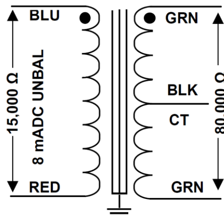
SCHEMATIC
